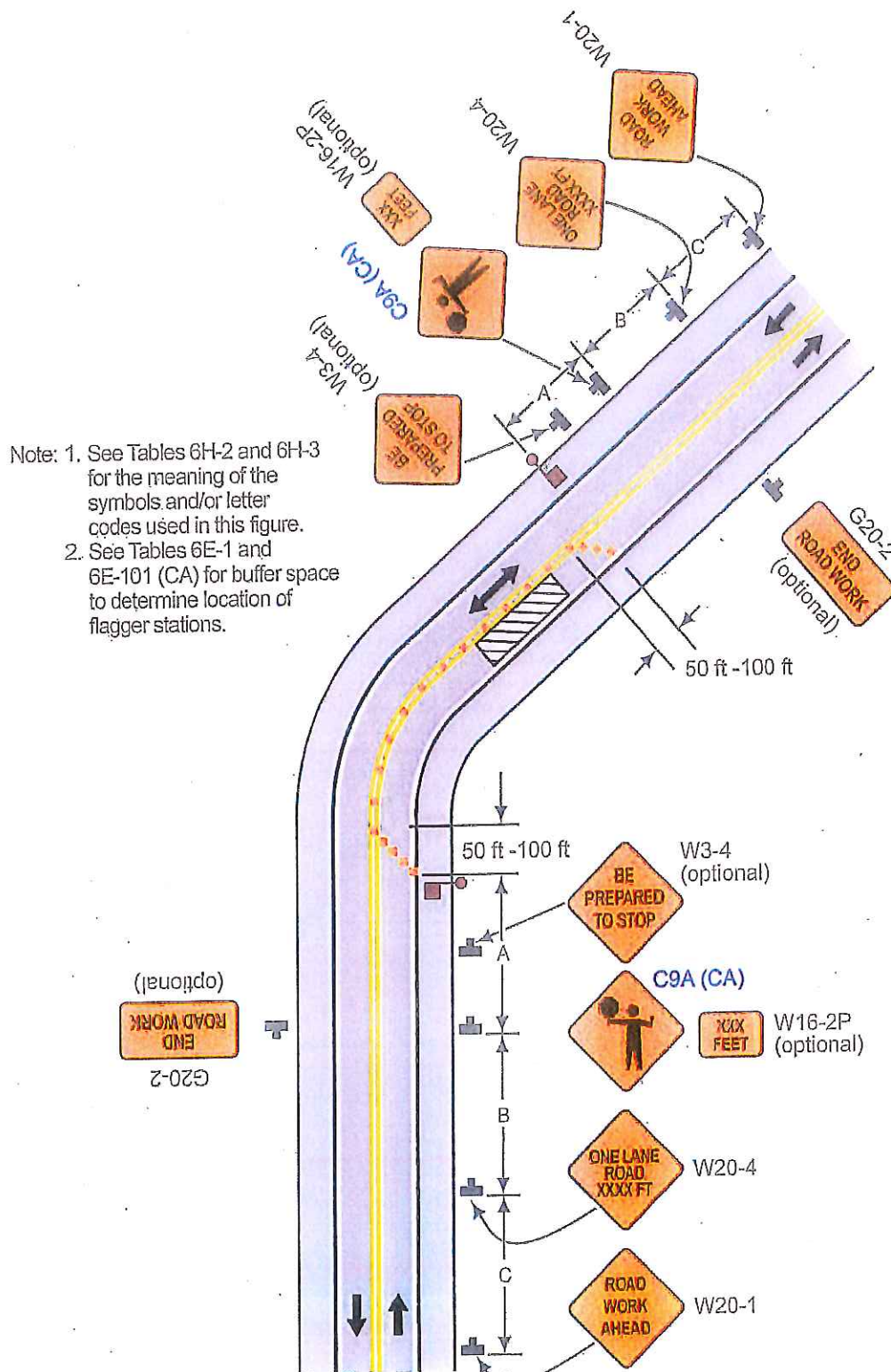
Typical Application 10
